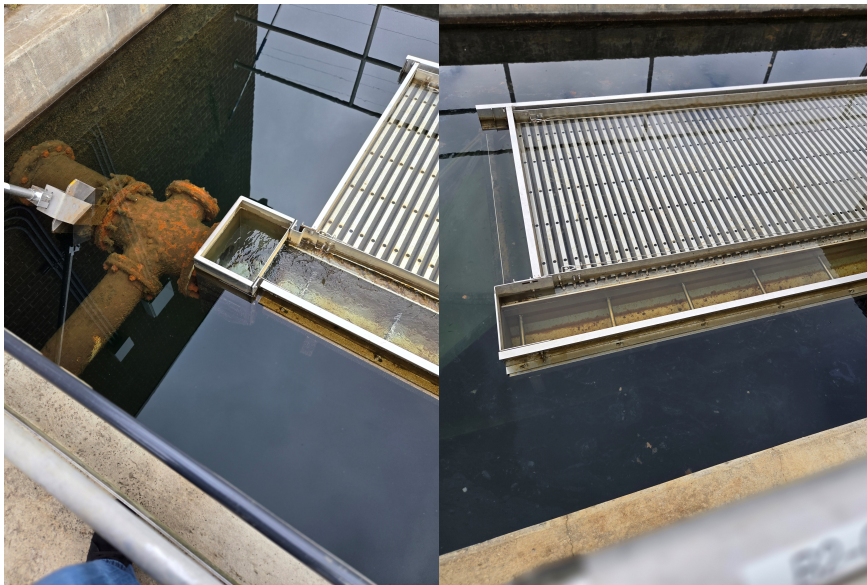
Plate Settlers and Collection Trough (to filters)
